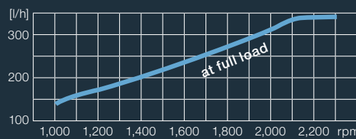
Fuel Consumption V12-1800
